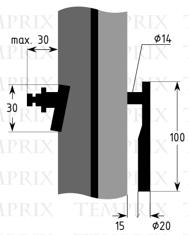
Detail X
